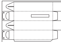
Wine Bottle Box (Window) 3.23 x 3.23 x 13.125
